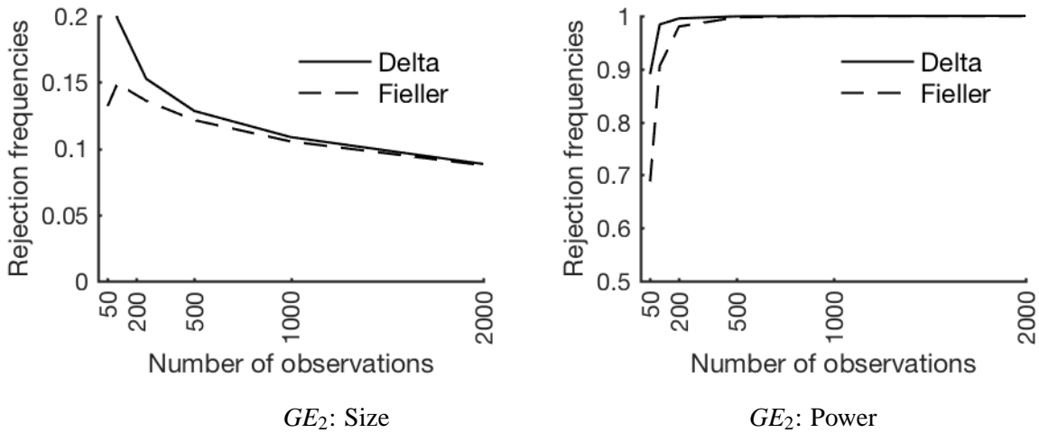
Figure 2: Size and power of Delta(-method) and Fieller-type tests for GE_2 index H_0: GE_2(X) = 0.71578 Left panel DGP: SM_X(a_X = 1.1, q_X = 4.327273) . GE_2(X) = 0.71578 Right panel DGP: SM_X(a_X = 1.7, q_X = 2.8) . GE_2(X) = 0.33503
